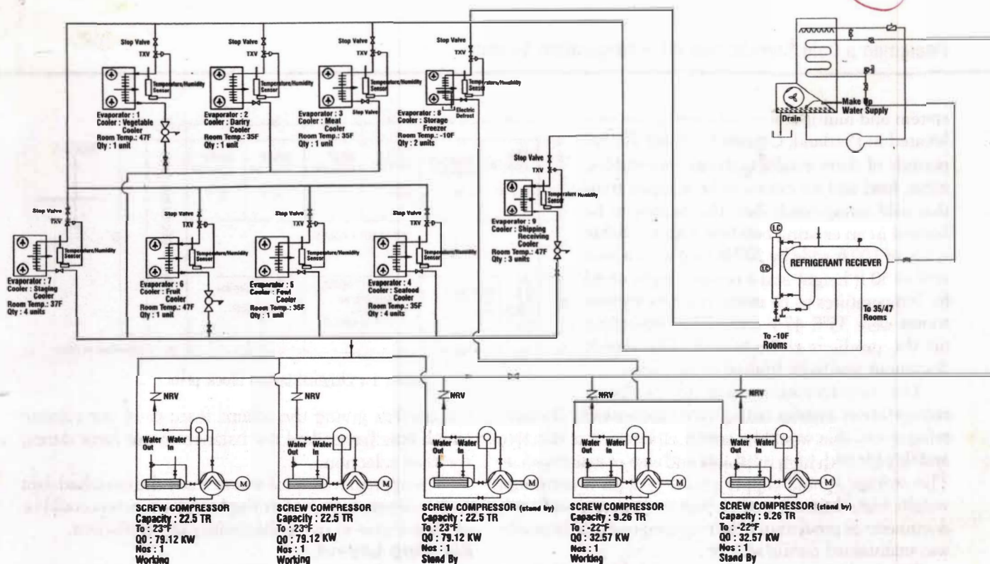
Figure 3: General refrigerant piping arrangement.
