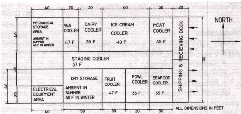
Figure 2 : Modified layout block plan.
