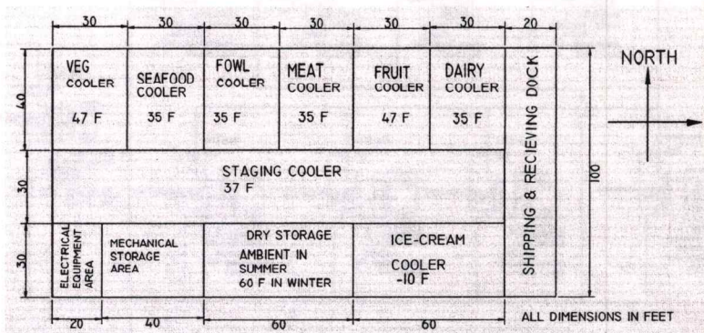
Figure 1 : Original layout block plan.
